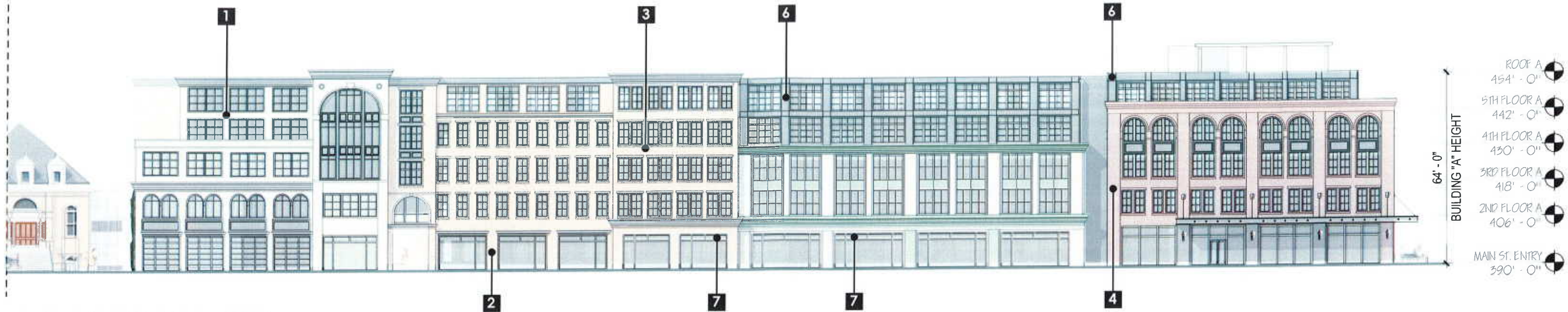
MAIN STREET ELEVATION
